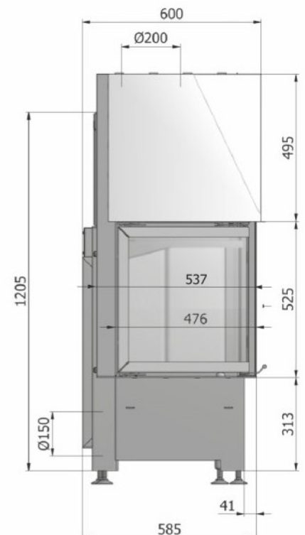
VOLCANO WPh 12
